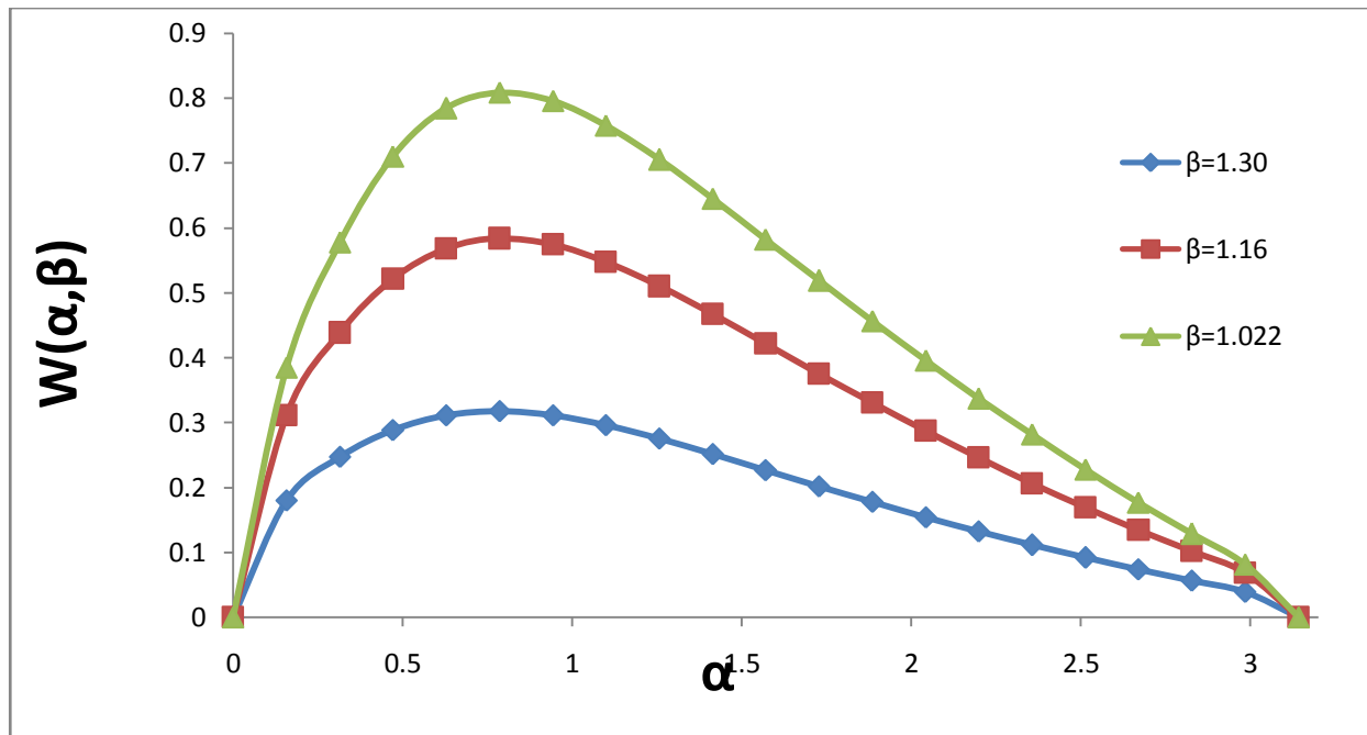
Fig.(2) velocity field W(\alpha, \beta) versus \alpha at different values of \beta when the outer sphere rotate with angular velocity \Omega and the inner sphere at rest for radii are R_1 = 2\text{cm} , R_2 = 4\text{cm} and the distance between two poles c=4\text{cm} .
