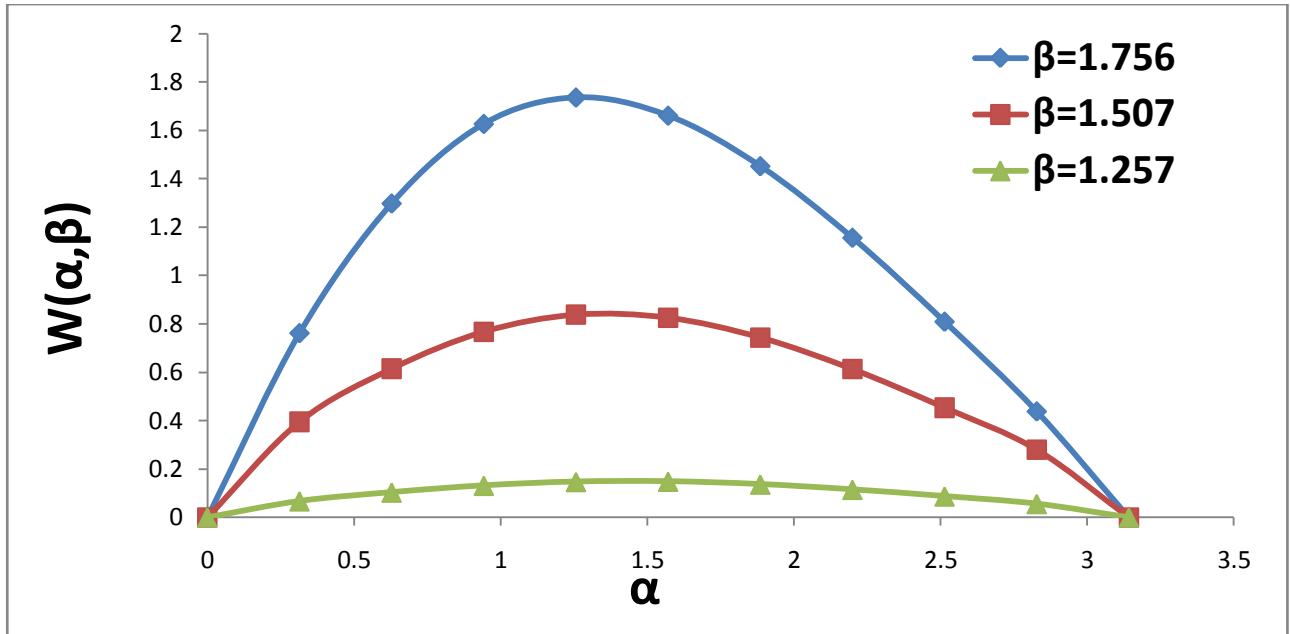
Fig.(4) velocity field W(\alpha, \beta) versus \alpha at different values of \beta when inner sphere rotate with angular velocity \Omega and outer sphere at rest for radii are R_1 = 2\text{cm} , R_2 = 4\text{cm} and distance between two poles c=4\text{cm} .
